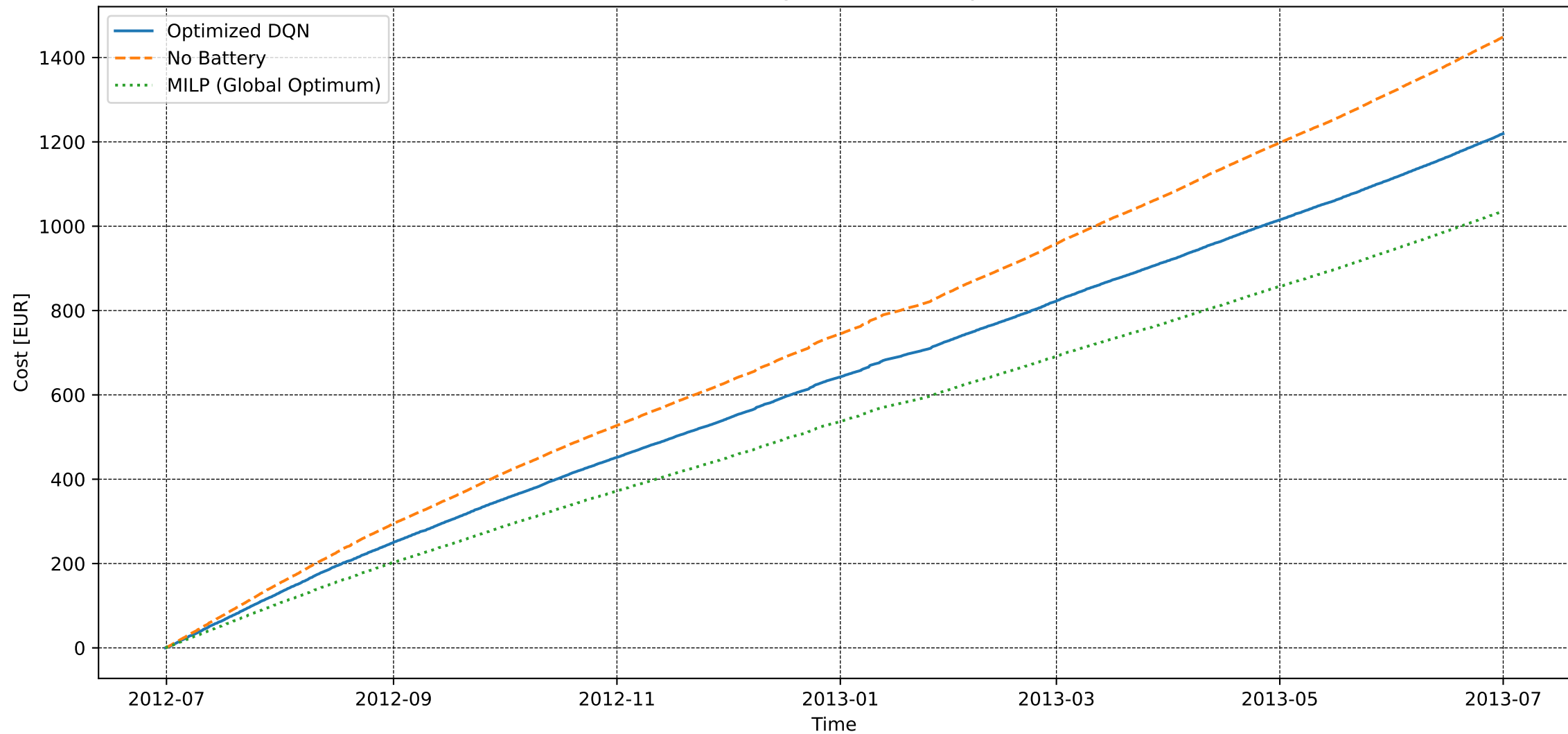
User 156 - Extended Convergence - Electricity Cost [DQN vs MILP]
